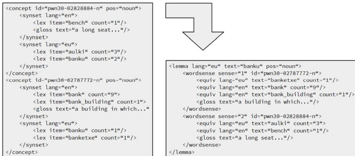
Figure 2: XML transformation
