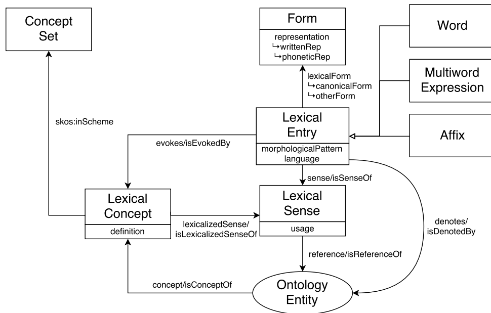
Figure 1: The Core OntoLex-Lemon Model
